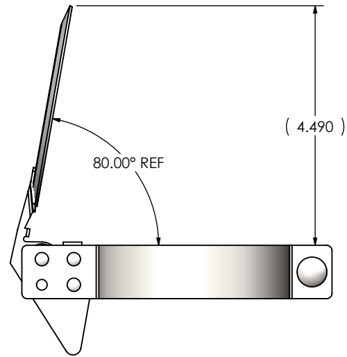
OPENED VIEW
