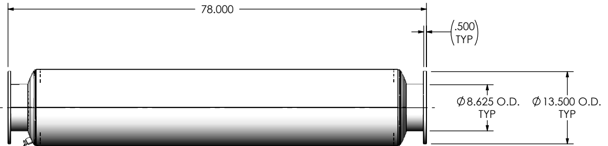
RIGHT VIEW
