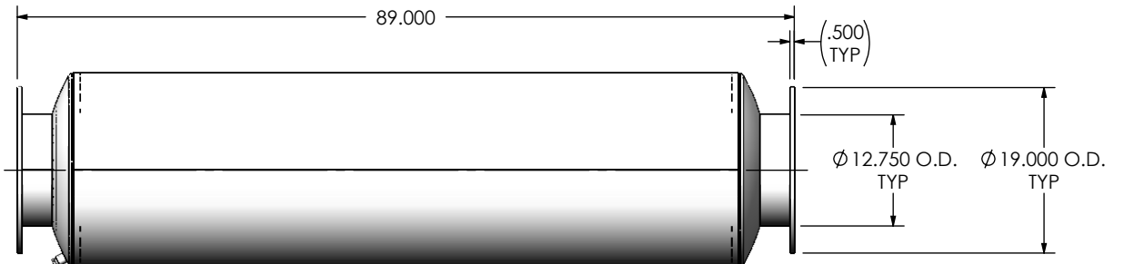
RIGHT VIEW
