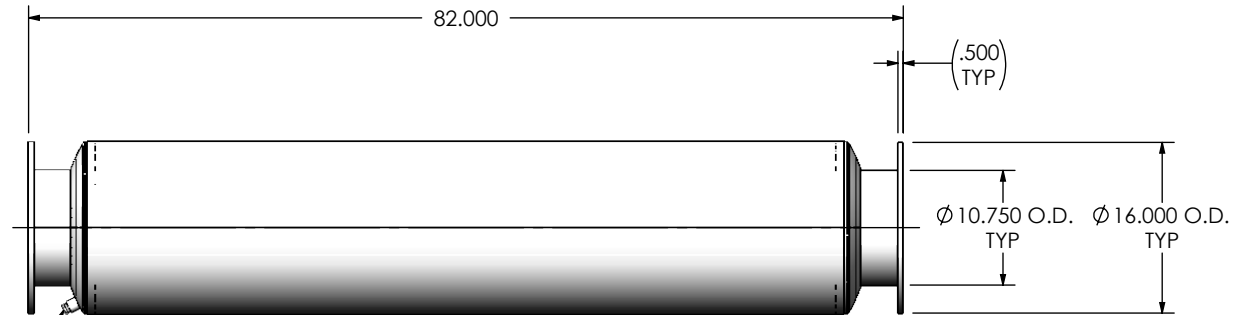
RIGHT VIEW
