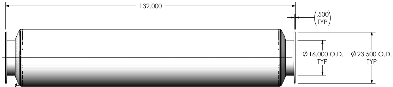
RIGHT VIEW
