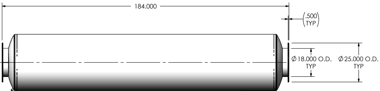
RIGHT VIEW
