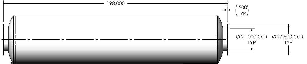
RIGHT VIEW
