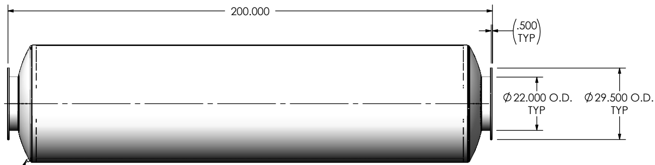
RIGHT VIEW
