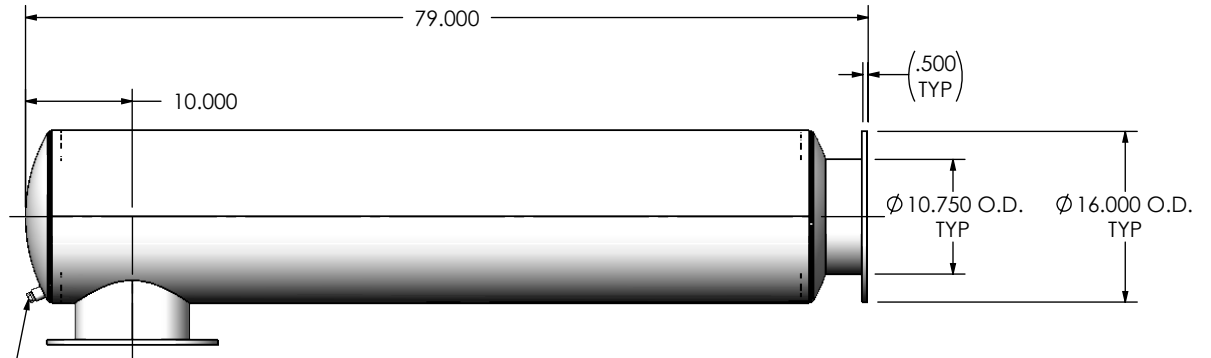
RIGHT VIEW
