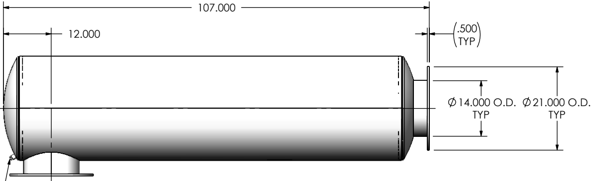
RIGHT VIEW
