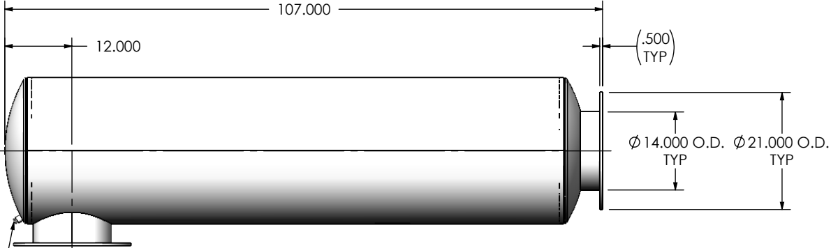
RIGHT VIEW
