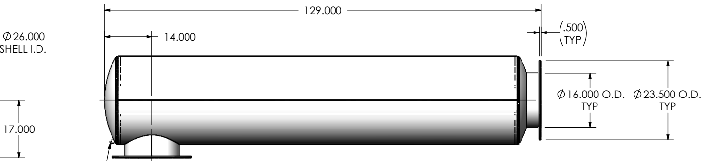
RIGHT VIEW
