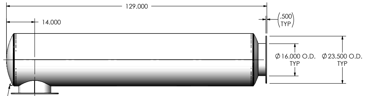
RIGHT VIEW
