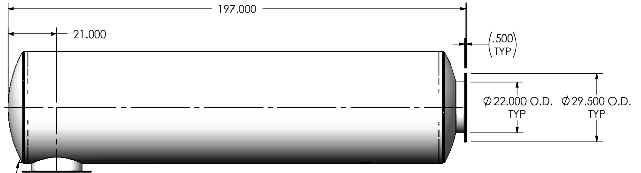
RIGHT VIEW
