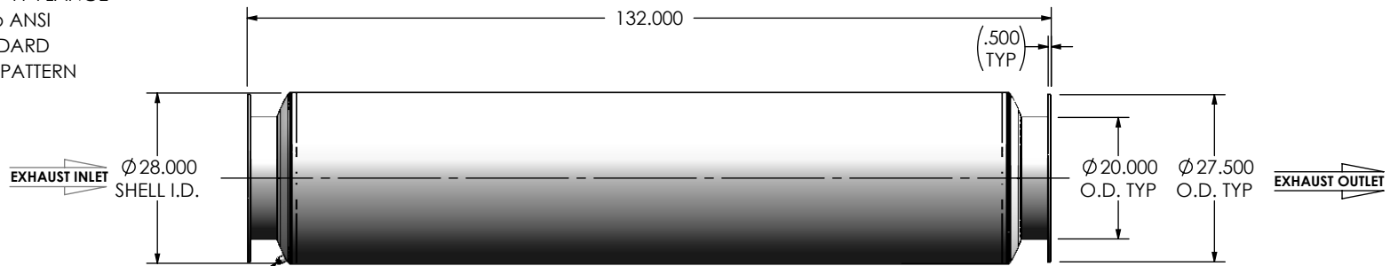
RIGHT VIEW
