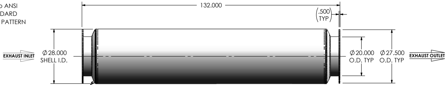
RIGHT VIEW
