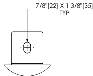
DETAIL A SCALE 1 : 7
