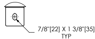
DETAIL A SCALE 1 : 12
